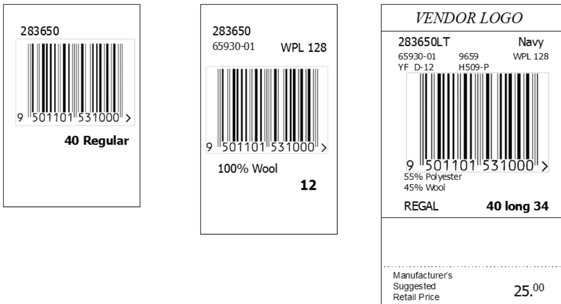
Figure 6.5.3.2-1. Vertical layout
